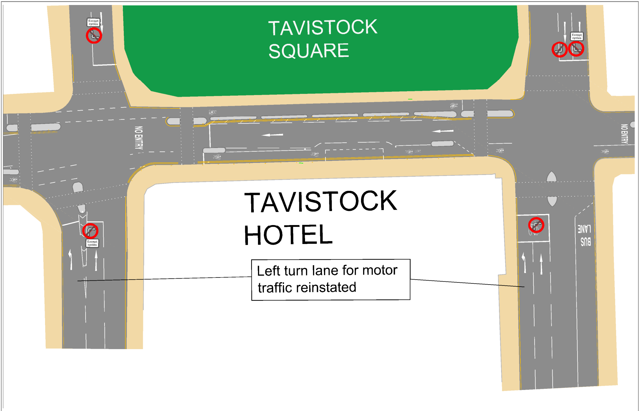
Drawing 2a: Proposals at Bedford Way and Woburn Place junctions with Tavistock Square
